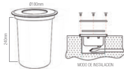
SPOT PISO CILINDRO ACERO 100-240v Ref.: BU6301
